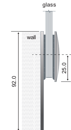
TOP VIEW
