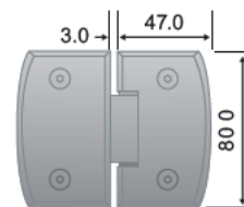
PANEL CUT OUT DOOR CUT OUT
