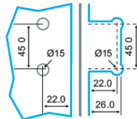
PANEL CUT OUT DOOR CUT OUT
