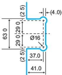
GLASS CUT OUT
