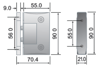
GLASS CUT OUT
