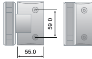
GLASS CUT OUT
