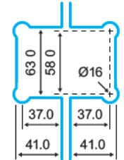
GLASS CUT OUT
