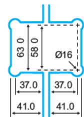
GLASS CUT OUT
