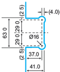
GLASS CUT OUT
