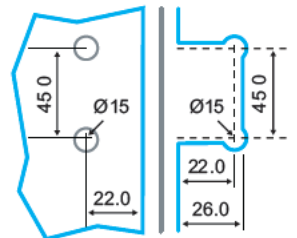
PANEL CUT OUT DOOR CUT OUT
