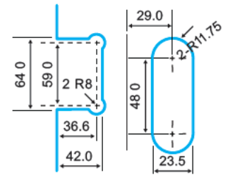
GLASS CUT OUT FIXED PANEL
