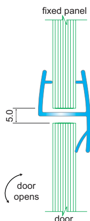
TOP VIEW
