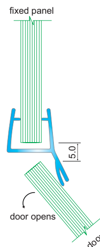
TOP VIEW
